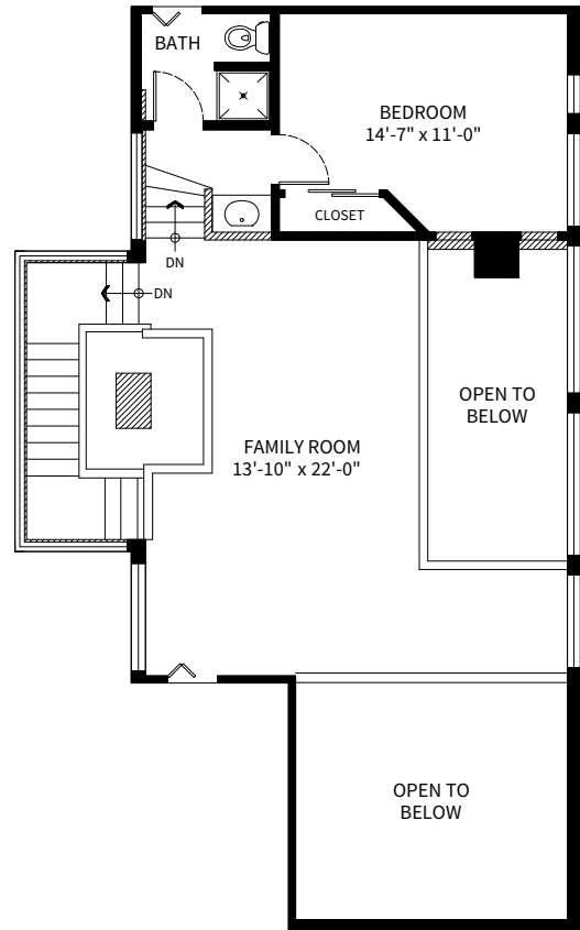
UPPER FLOOR PLAN Ceiling Height: 13'-10" Vaulted Ceiling
